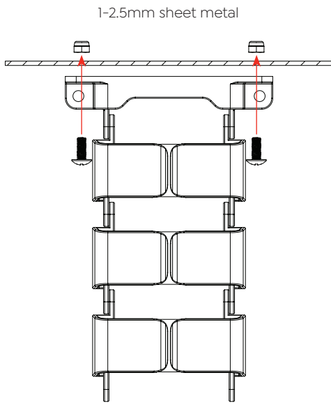
Cable tray mounting
