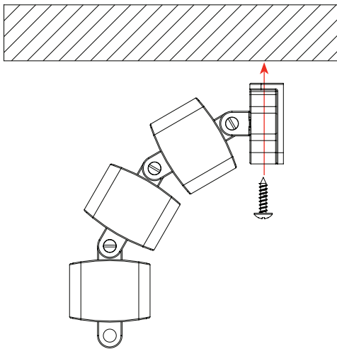
Under worktop mounting
