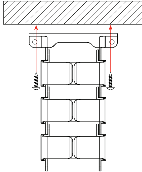
Under worktop mounting
